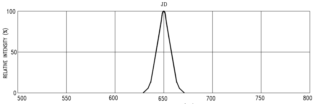
Fig1. Spectral Emission
