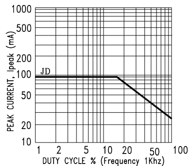
Fig5. Maximum Peak Current vs. Duty Cycle %
